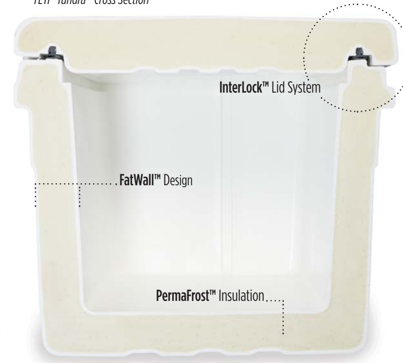
YETI® Tundra™ Cross Section
